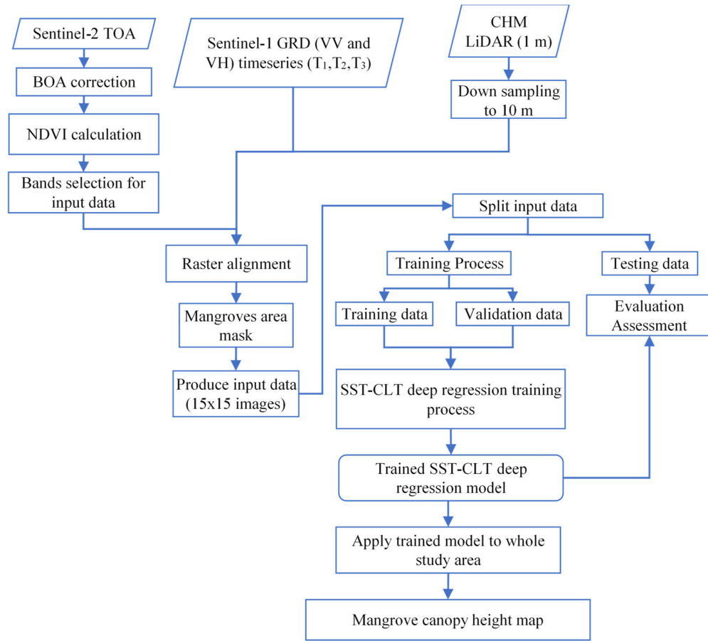
Fig. 1. Processing flowchart of this study. TOA, top of atmosphere; BOA, bottom of atmosphere; NDVI, normalized difference vegetation index; and CHM, canopy height model.
