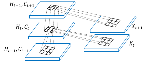
Fig. 5. Inner structure of the 2DConvLSTM network [44].
