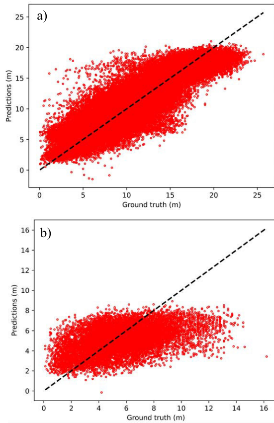
Fig. 8. Scatter plot of the ground-truth LiDAR CHM data (testing data) versus the prediction results: (a) ENP and (b) CHPSP.
