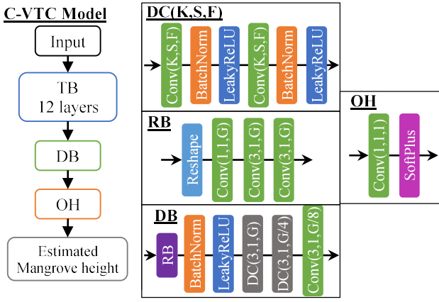
Fig. 7. Implementation of C-VTC with G = 512 inspired by Fayad et al. [47]. TB stands for vision-transformer block, DC (K, S, F) stands for deep convolutional (kernel, stride, and filters), RB stands for reshape block, DB stands for decoder block, and OH stands for output head.
