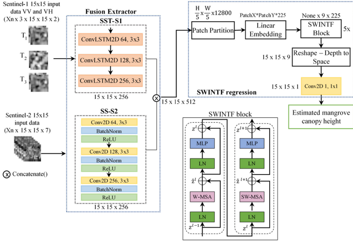
Fig. 6. Architecture of the proposed SST-CLT deep regression model.
